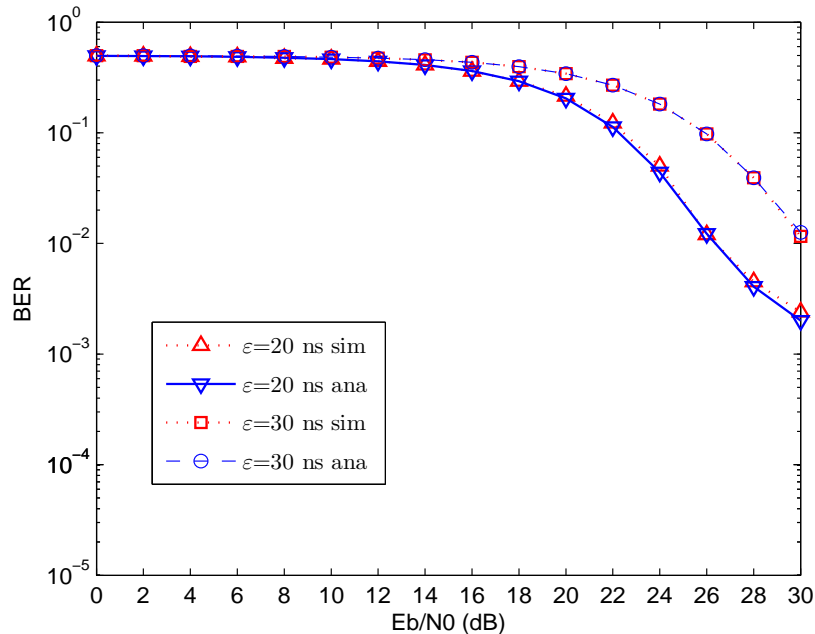
Figure 79: BER performance of PWM in multipath channels (CM4 model, \delta = D = 80 ns, \varepsilon = 20 and 30 ns)
