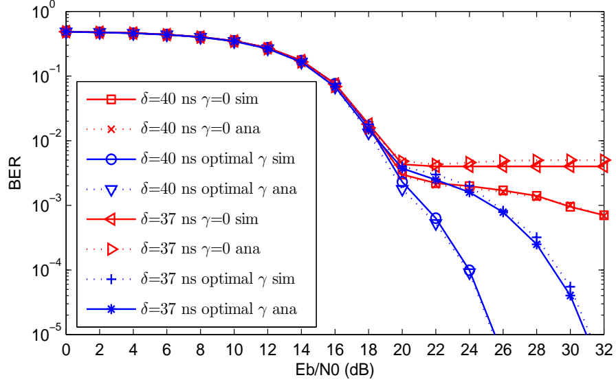
Figure 47: Comparison of BER performance of 0 and optimal threshold PPM systems in multipath channels(CM4 model, D=80 ns, \delta =40 and 37 ns)
