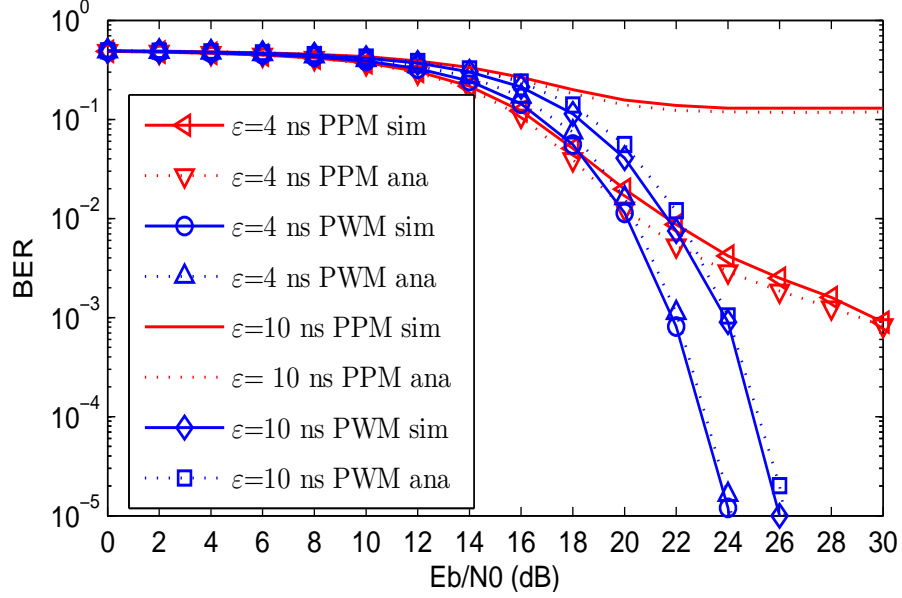
Figure 21: Comparison of BER performance of PWM and PPM in the presence of synchronization errors(CM4 model, \delta = D = 80 ns, \epsilon = 4, 10 ns).
