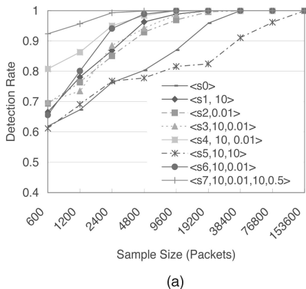
Fig. 4. Detection rate for link-based batching. (a) Mutual information. (b) Matched filter.
