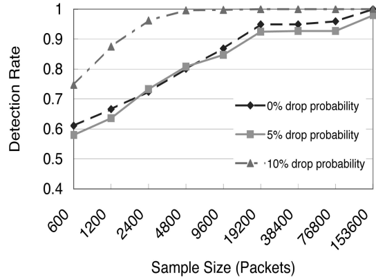
Fig. 8. Detection rate for network with packet loss.
