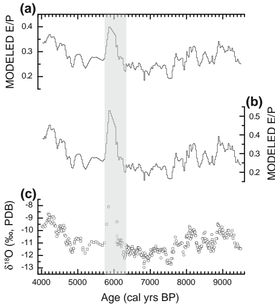
Fig. 9 Comparison of \delta^{18}\text{O} records with modeled E/P results for Ahung Co. a Modeled E/P time series from \delta^{18}\text{O} records of sedimentary carbonates in Ahung Co. b Modeled E/P results using an isotopic mass balance approach (Gonfiantini 1986; Gibson and Edwards 2002), E/P = (\delta_I - \delta_L)/(\delta_E - \delta_L) , where subscripts denote inflow (I), lake (L), and evaporation (E). c Carbonate \delta^{18}\text{O} records from lake sediments (Core 2A: open squares; Core 3A: open circles) of Ahung Co, central Tibet (Morrill et al. 2006). \delta^{18}\text{O} of paleolake water ( \delta_w ) is deduced from \delta^{18}\text{O} of sedimentary carbonates ( \delta_c ), using T = 16.0 - 4.14 (\delta_c - \delta_w) + 0.13(\delta_c - \delta_w)^2 (Anderson and Arthur 1983), where T is water temperature ( 22.5^\circ\text{C} ) when carbonate forms (Galat and Jacobson 1985). Note that \delta^{18}\text{O} values of lake inputs are assumed to be similar to those of Cona Lake
