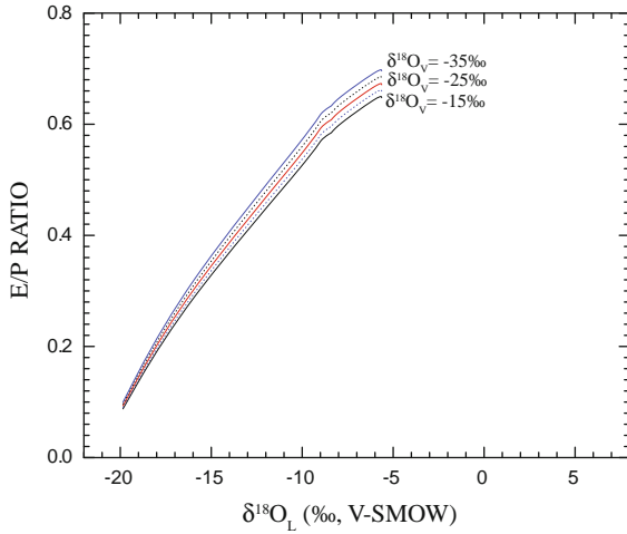
Fig. 7 Modeled E/P sensitivity to the isotope composition of free atmospheric vapor
