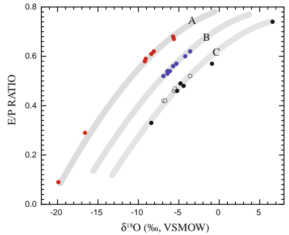
Fig. 8 Plot of modeled E/P ratio versus \delta^{18}\text{O} of lake water ( \delta^{18}\text{O}_L ). Lines A, B, and C represent generalized relationships of modeled E/P and \delta^{18}\text{O}_L , corresponding different \delta^{18}\text{O} of lake inputs ( \delta^{18}\text{O}_I ). \delta^{18}\text{O}_I values for Lines A, B, and C are -21.3 , -17.5 , and -15.3\text{‰} . Red filled circles denote Class I lakes, blue filled circles denote Class II lakes, black filled circles denote Class III lakes, and open circles denote Class IV lakes
