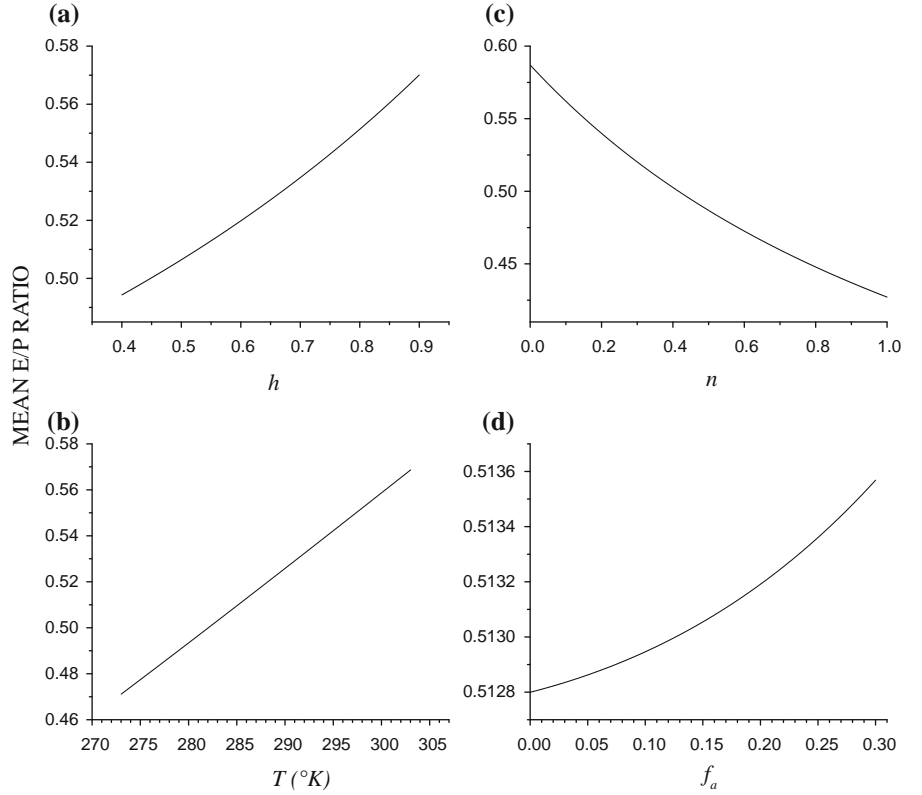
Fig. 6 Plots of sensitivity of model parameter values to the mean E/P ratio of Tibetan lakes. a Modeled E/P sensitivity to relative humidity. b Modeled E/P sensitivity to surface water temperature. c Modeled E/P sensitivity to molecular diffusion factor. d Modeled E/P sensitivity to the fraction of advected water vapor
