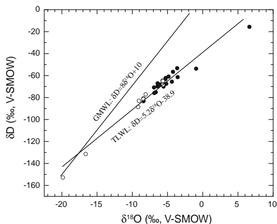
Fig. 2 Relationship of \delta^{18}\text{O} and \delta\text{D} in surface waters from open lakes (i.e. lakes with outlets) (open circles) and closed-basin lakes (filled circles) in the Tibetan Plateau
