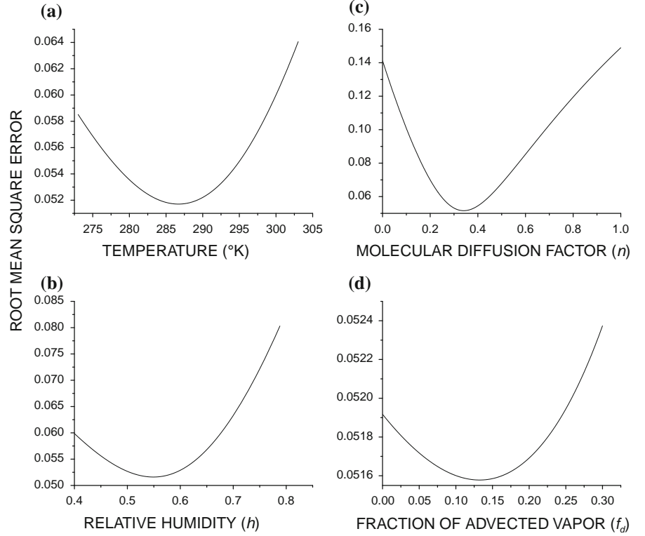
Fig. 5 Optimization of model parameter values of surface water temperature (a), relative humidity (b), molecular diffusion factor (c), and fraction of advected vapor (d). The optimization was based on the minimization of the root-mean-square relative error between \delta^{18}\text{O} -inferred E/P and \delta\text{D} -inferred E/P
