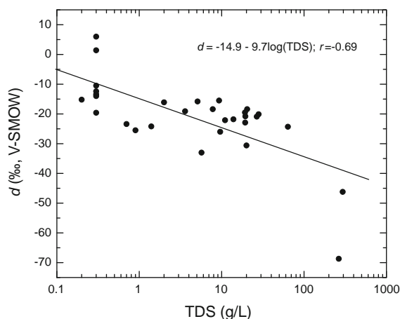
Fig. 3 Correlation of deuterium excess ( d ) and TDS in surface waters from Tibetan lakes
