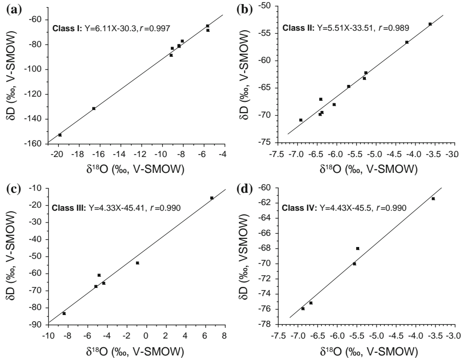
Fig. 4 Relationships between \delta^{18}\text{O} and \delta\text{D} in lake waters for Class I (a), Class II (b), Class III (c), and Class IV (d)
