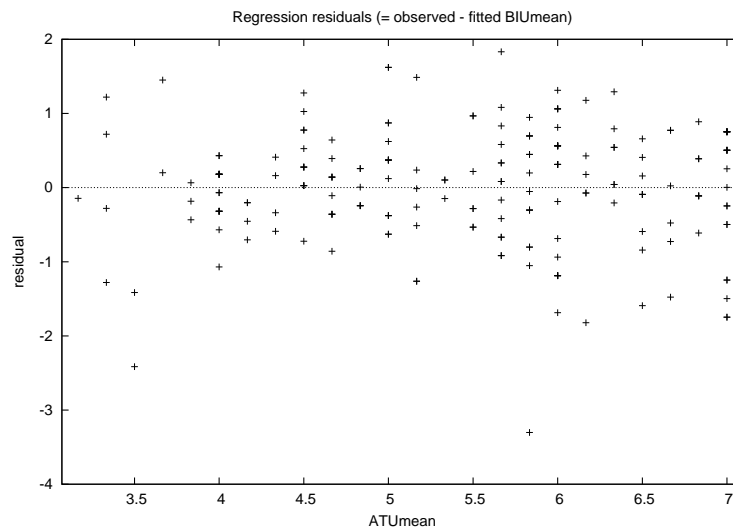
(b) Residuals versus Independent Variable (ATUmean)
