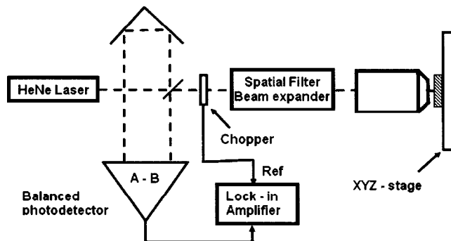
FIG. 8. Confocal setup with a balanced photodetector and lock-in detection.
