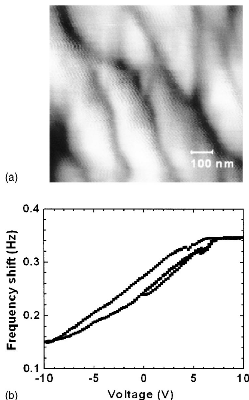
FIG. 9. (a) AFM image of a strain BaTiO 3 thin film grown on Si, taken at 10 K. (b) Piezoresponse signal obtained by cycling the voltage between the tip and the sample.
