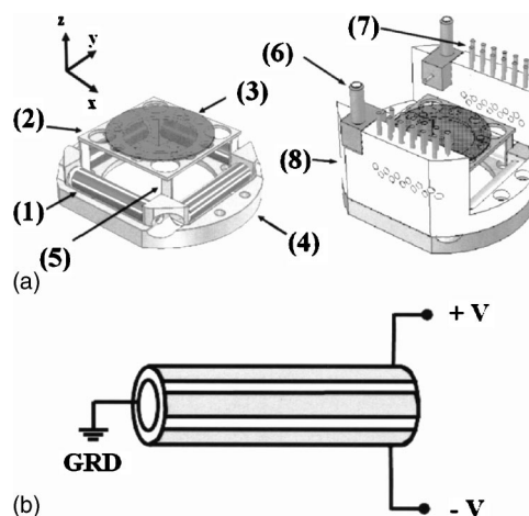
FIG. 3. (a) Perspective view of the XYZ stage. (1) Quadrant piezotubes, (2) titanium base, (3) sapphire sample plate, (4) Macor base, (5) L shaped titanium plates, (6) microwave connectors, (7) electrical pins, and (8) macor frame. (b) Opposite voltages applied to electrode pairs while the center electrode is grounded, bend the piezotube in the field direction.
