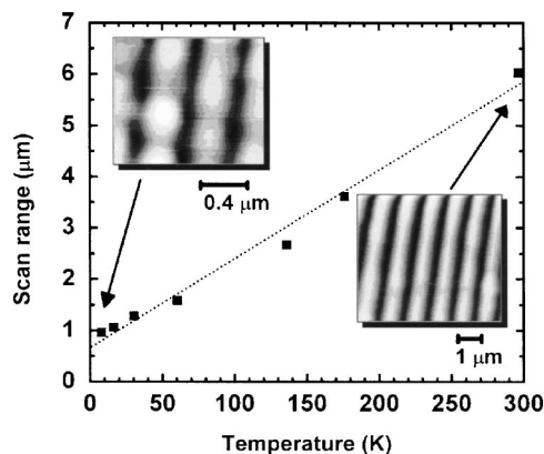
FIG. 6. Temperature performance of the XYZ stage.
