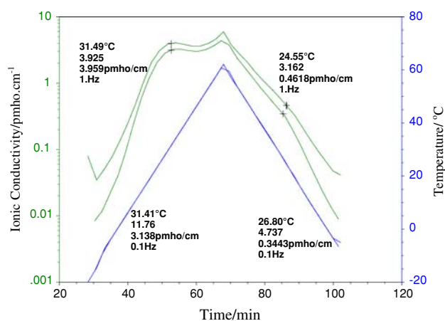
Fig. 4 Dielectric thermal analysis (DETA) of 40/60 mol% cholesterol PC film
