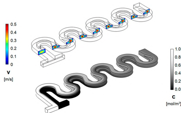
Figure 4. Velocity magnitude (cross-sectional maps) ( top ) and concentration distribution (surface map) ( bottom ) along the channel of a non-rectangular cross-section serpentine micromixer ( R_{in} = W/2 = 100 \text{ }\mu\text{m} , and Re = 20 ).
