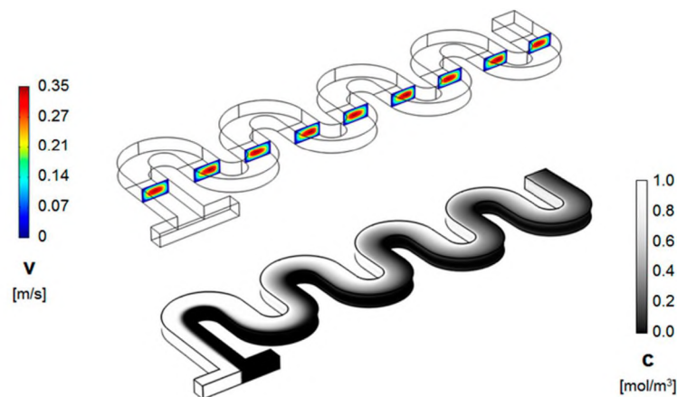
Figure 3. Velocity magnitude (cross-sectional maps) ( top ) and concentration distribution (surface map) ( bottom ) along the channel of a standard serpentine micromixer ( R_{in} = W/2 = 100 \text{ }\mu\text{m} , and Re = 20 ).
