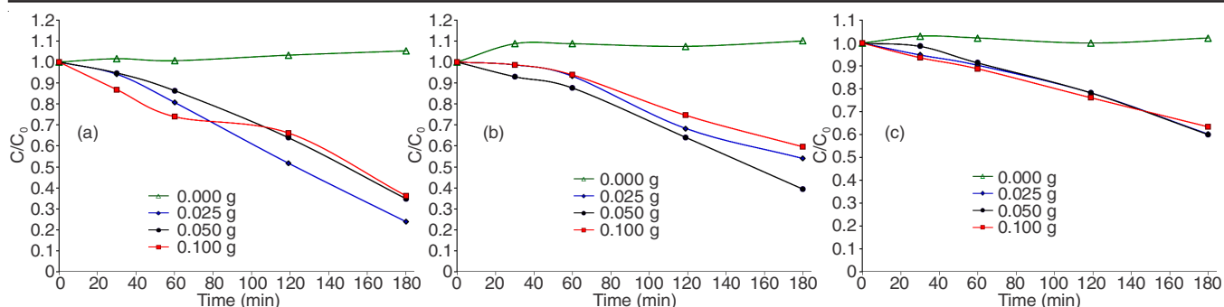
Fig. 6. Influences of doses of (a) Co-doped TiO 2 with an initial concentration of 24 mg/L, (b) Co-doped TiO 2 with an initial concentration of 34 mg/L and (c) Co-doped TiO 2 with an initial concentration of 44 mg/L, as monitored by changes in the absorbance at 484 nm: (a) Control; (b) 0.025 g; (c) 0.050 g; (d) 0.100 g
