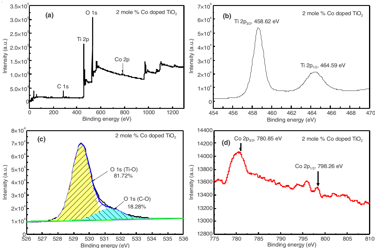
Fig. 3. XPS spectra of the 2 mole % Co-doped TiO 2 : (a) wide-survey spectrum; (b) Ti 2p core level spectrum; (c) O 1s core level spectrum; (d) Co 2p spectrum
