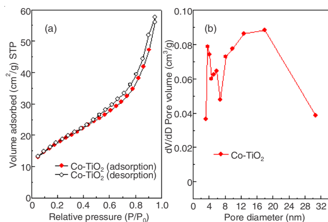
Fig. 4. (a) Nitrogen adsorption-desorption isotherms and (b) BJH pore size distributions of 2 mole % Co-doped TiO 2 powder
