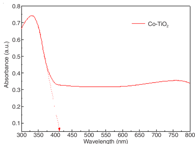
Fig. 5. UV-visible absorption spectra of 2 mole % Co-doped powder prepared by solid state reaction technique
