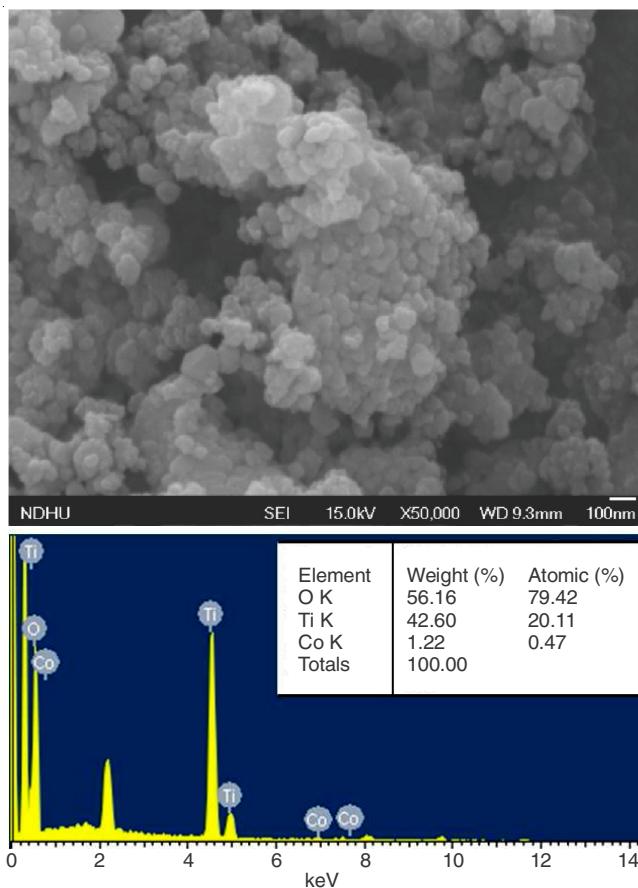
Fig. 2. SEM images and EDS results of 2 mole % Co-doped TiO 2 spectra of the 2 mole % Co-doped TiO 2
