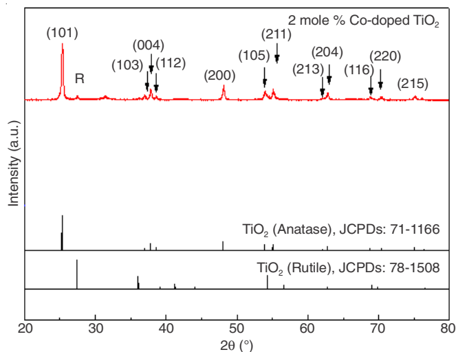
Fig. 1. XRD pattern of 2 mole % Co-doped TiO 2 prepared by solid state reaction technique
