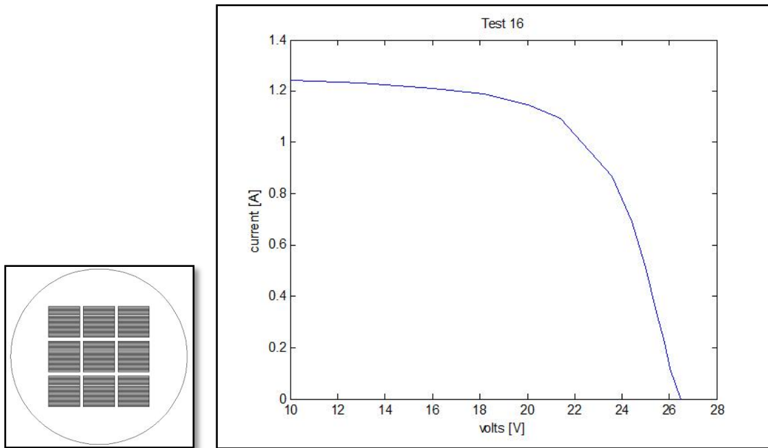
Figure 64: Square Receiver at 30 % Fill, 23 Watts P_{mp}
