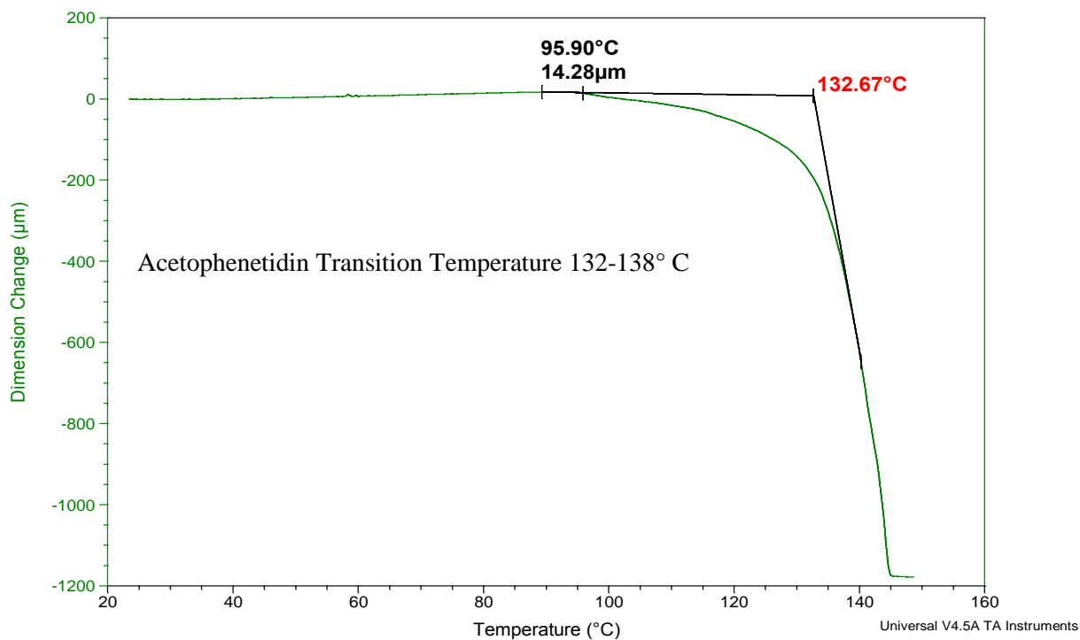
Figure 28 TMA of Acetophenetidin curve showing extrapolated onset melt temperature.
