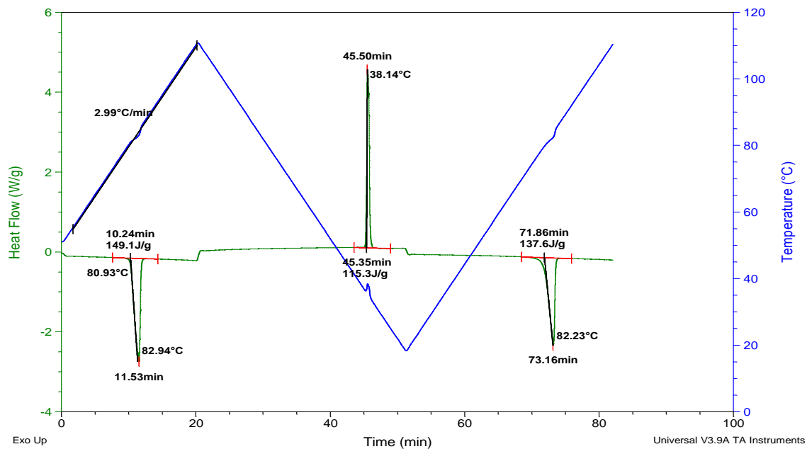
Figure 22 Vanillin DSC curve showing Tmp (83 °C), Tc (38 °C), Heat of fusion (149 J/g) for first endothermic peak and (138 J/g) for second endothermic peak and Heat of crystallization (115 J/g).
