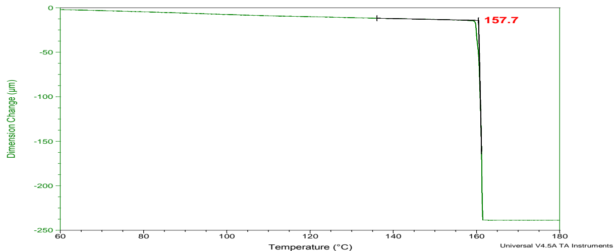
Figure 16 TMA Curve of Indium
