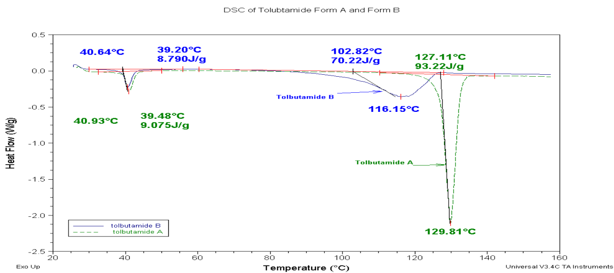
Figure 13 DSC of Polymorphs of Tolbutamide: Tolbutamide A (Form 1) and B (Form 3)
