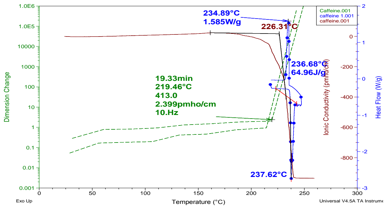
Figure 19 Caffeine run by TMA (solid line), DSC (dotted line) and DEA (dashed line).
