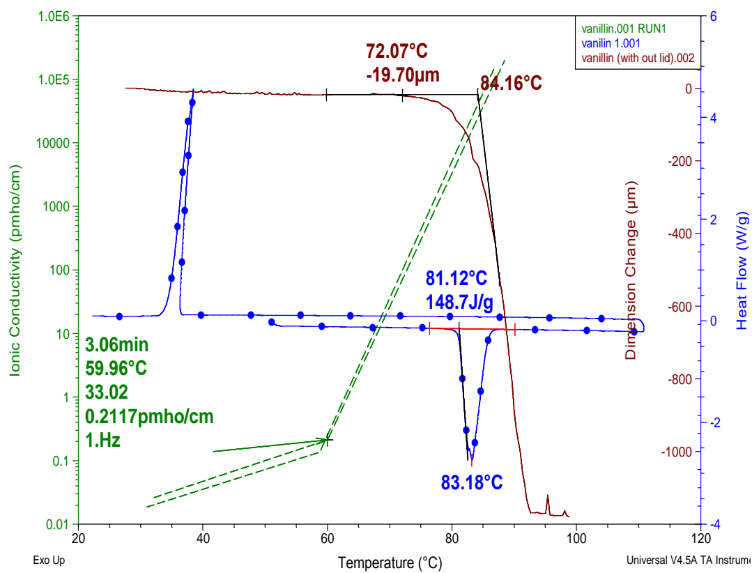
Figure 18 Vanillin run by TMA (solid line), DSC (dotted line) and DEA (dash line).
