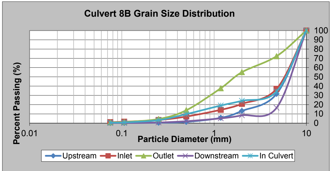
Figure 5.4 Culvert 8B Grain Size Distribution
