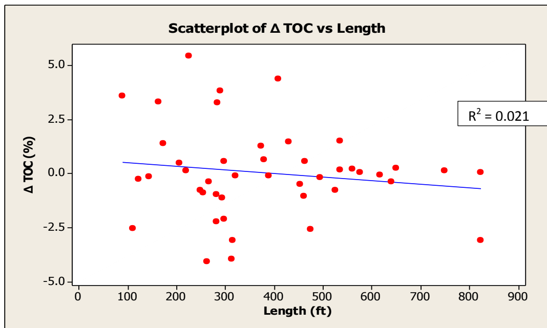
Figure 5.5 Scatterplot of \Delta\text{TOC} vs Length in All Culverts
