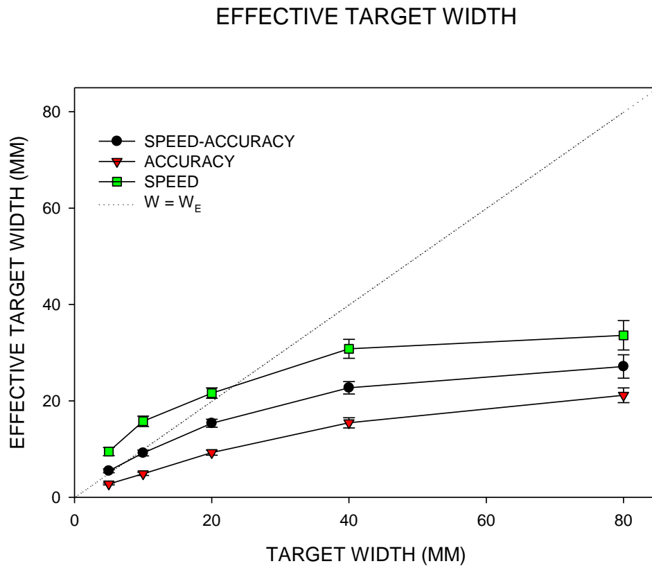
Figure 5. Effective target width as a function of target width. The dotted line indicates the point at which effective target width and target width is equivalent. Data points above the line indicate that effective target width is larger than target width. Data points below the line indicate that effective target width is smaller than target width.
