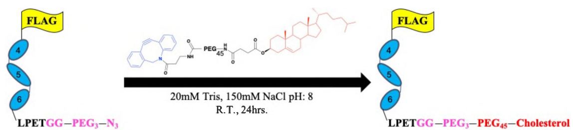
Figure 4.7: Copper free click chemistry addition of DBCO-PEG 2000 -Cholesterol to rTM 456 -azide
