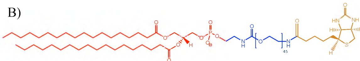
Figure 3.1: Structures of Cholesterol-PEG 2000 -Biotin and DSPE-PEG 2000 -Biotin
