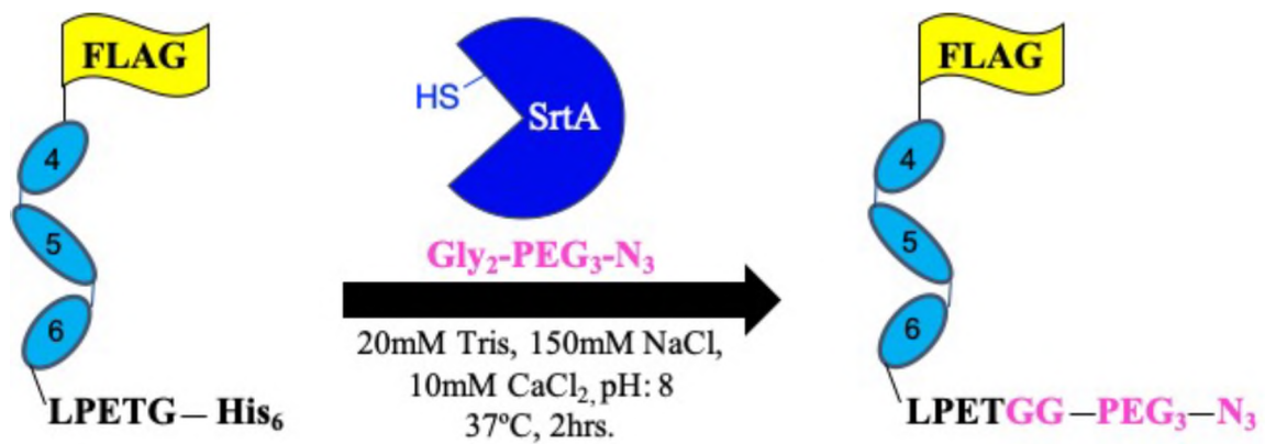
Figure 4.5: Sortase A Ligation Scheme
