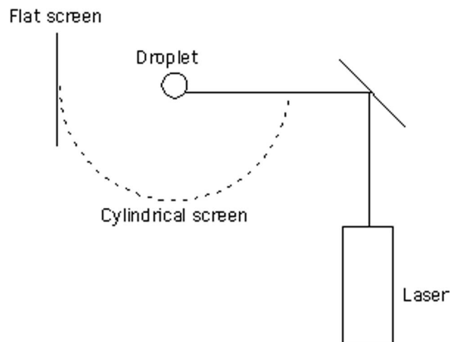
Fig. 7. Experimental apparatus for photographing external reflection caustics in the laboratory. The flat viewing screen was used for looking at caustics in the near-0° scattering direction; the semi-cylindrical screen was used to examine the caustics from 0° to 180°.
